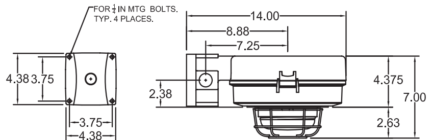
Wall mount with threaded glass globe and guard.
