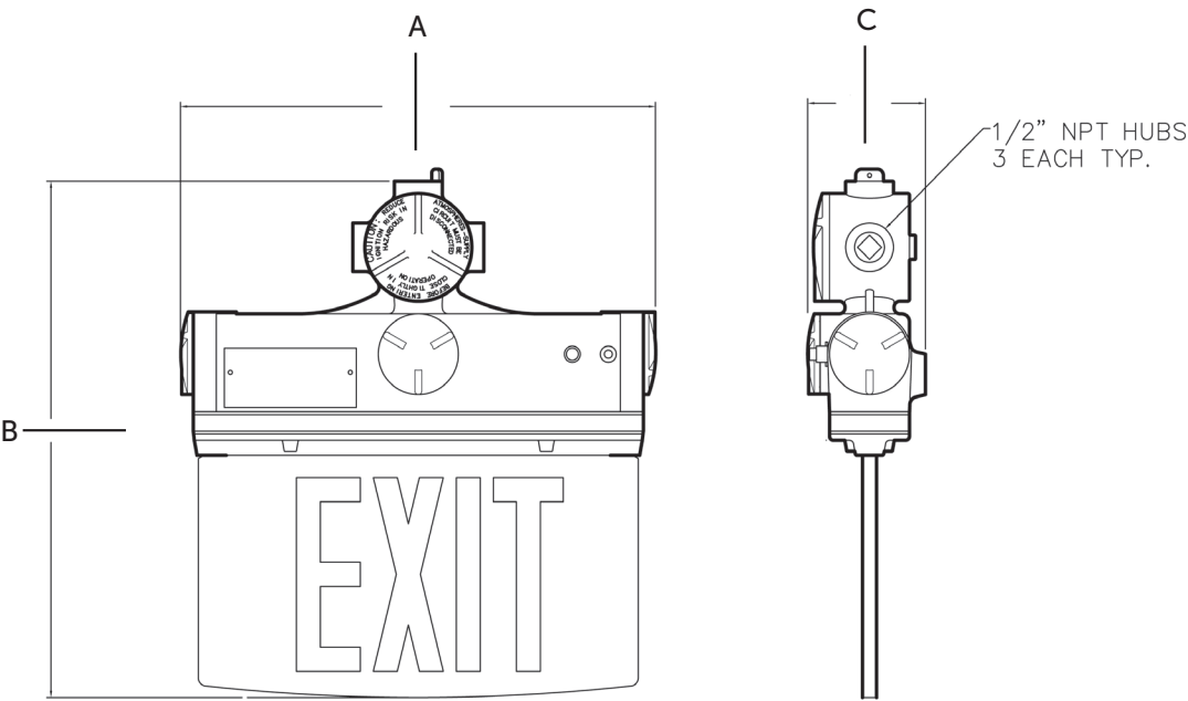
HLS Series Fixture Dimensions (inches)
