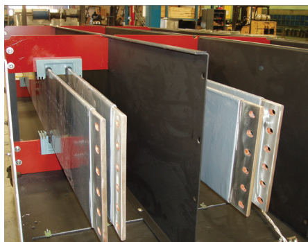
Avail Segregated Phase Bus Systems are designed for the application or user preference for decades of reliable service.
