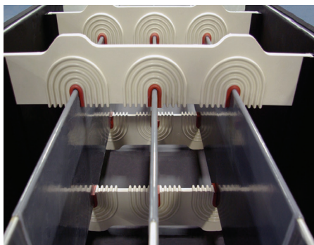
Avail Non-Segregated Phase Bus Systems provide proven cost-effective performance, low maintenance, and ensure greater reliability.
